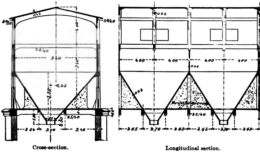
FIG. 323.—Sawdust bins of the Waldhof Pulp Mill.
