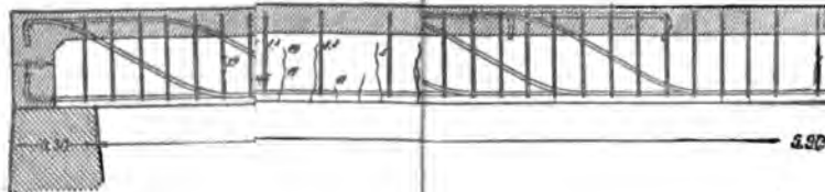
FIG. 185.—Continuous beams but with \frac{1}{2} in. approx. in diameter.
