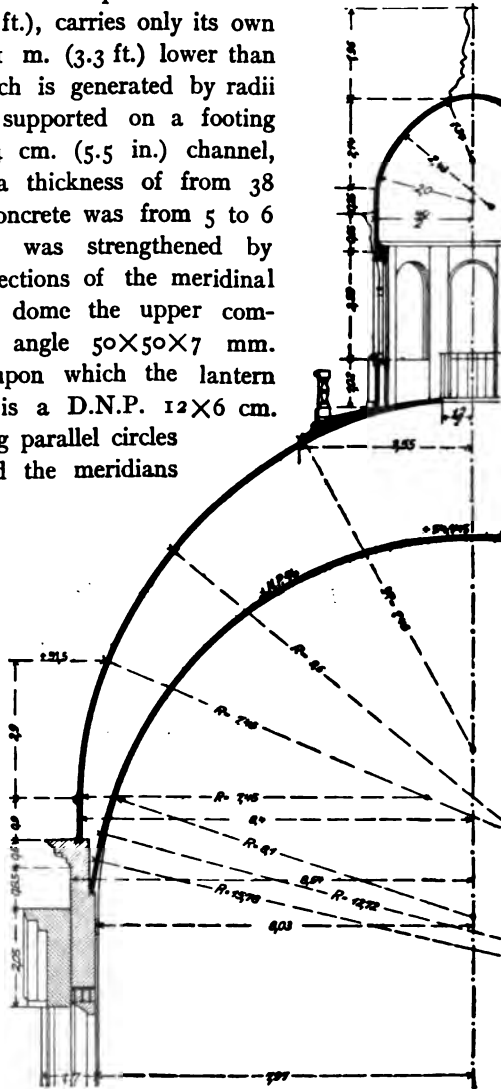
FIG. 252.—Vertical section through the cupola of the Army Museum in Munich.
