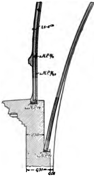
FIG. 251.—Detail of base of cupola.
