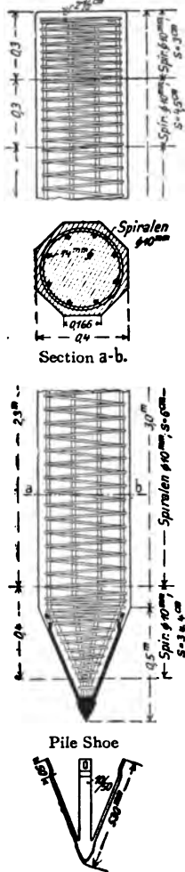
FIG. 264. — Reinforced concrete pile for the top of the canal in Mülhausen in Alsace.
