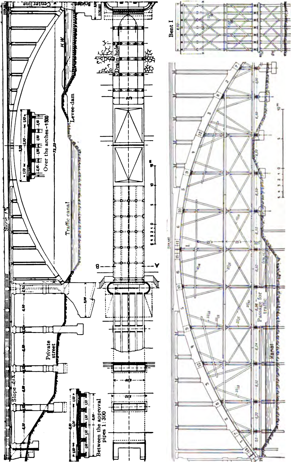
FIG. 296.—Isar Bridge near Grünwald. Longitudinal section, ground plan and centering for the left span.
