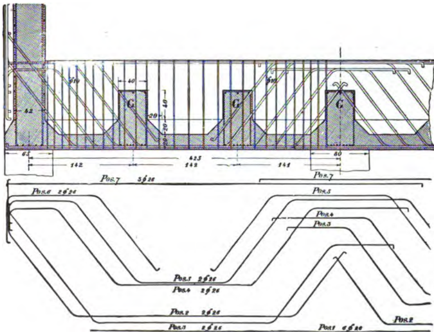
FIG. 326.—Välklingen coal pockets. Details of the rods in the girders in the bottoms.
