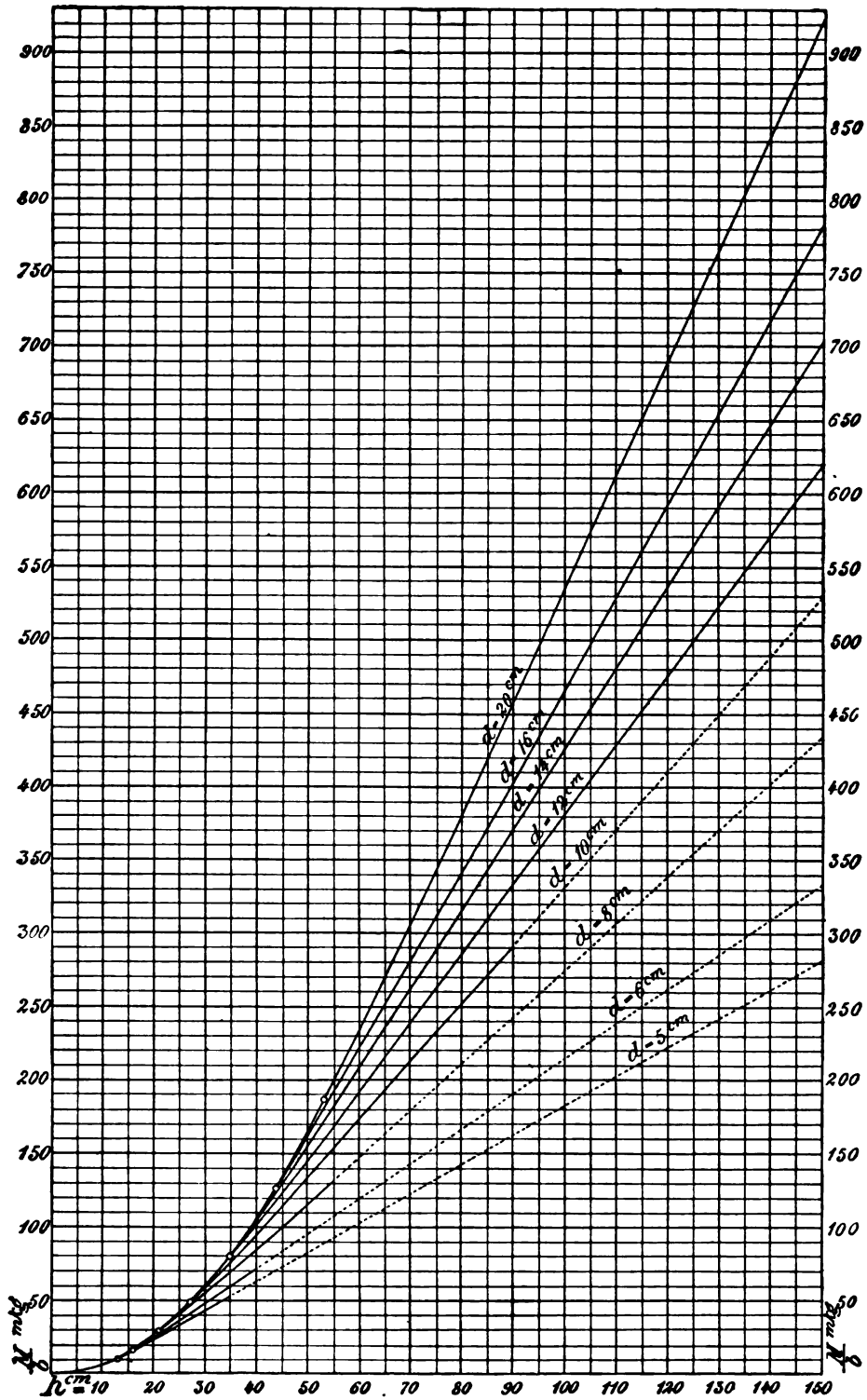
FIG. 103.—Diagram showing the relation between h and \frac{M}{b} in T-beams for various slab thicknesses d , and stresses \sigma_s = 1000 \text{ kg/cm}^2 , and \sigma_b = 40 \text{ kg/cm}^2 (14,220 and 569 lbs/in 2 ).
