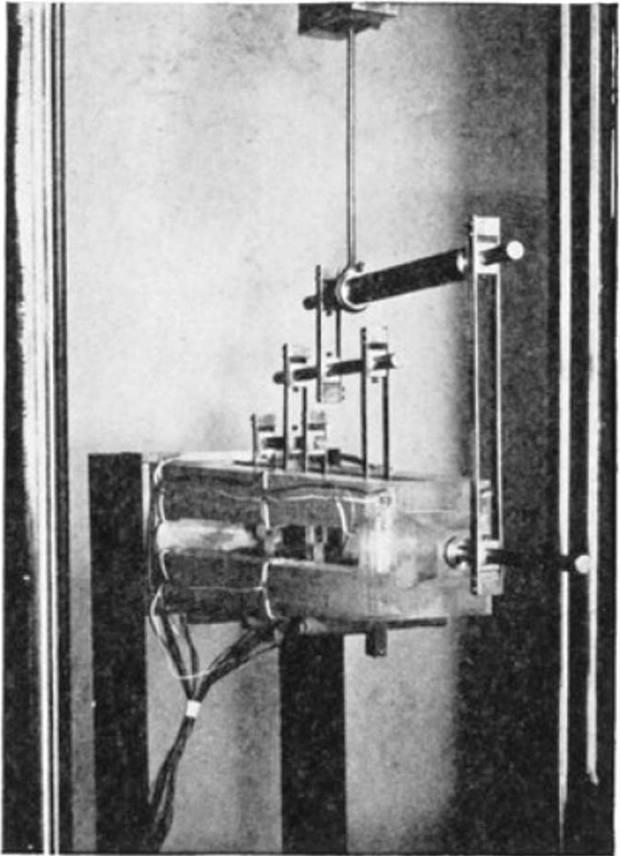
Fig. 5. Perspex model (laid horizontally), to the scale of 1/200 , of a monument about 100 m. high to be built in concrete. Electric strain gauges were used for both static and dynamic strain measurements
