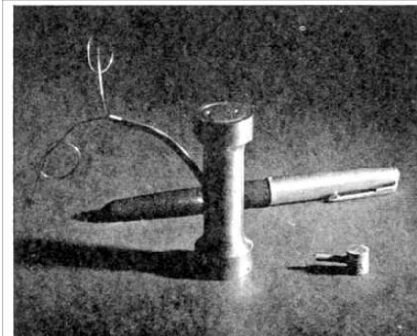
Fig. 10. Small magnetostriction cells to be left inside models for direct stress measurements
