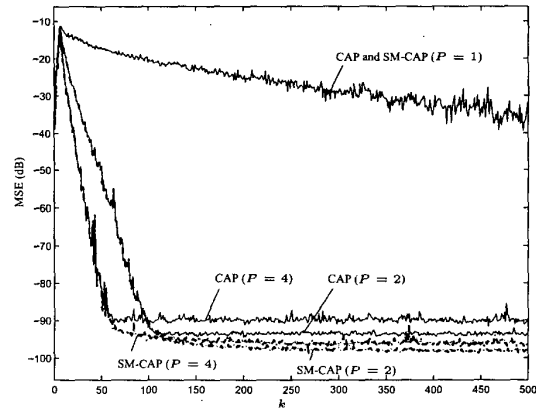
Fig. 1. Learning curves for the CAP and the SM-CAP algorithms with P = 1 , P = 2 , and P = 4 data reuses, \sigma_n^2 = 10^{-10} , \gamma = 3\sigma_n , and colored input signal.
